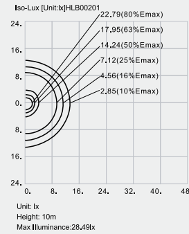
Lux-Distance Curve
