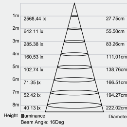
Lux-Distance Curve
